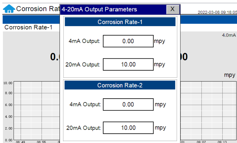
Figure 16 - 4-20mA setting
