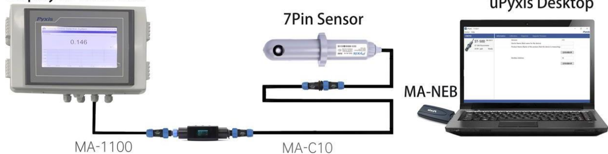
Figure 8. Connect the ST-540 series to a computer via MA-NEB and MA-WB Bluetooth adapters
