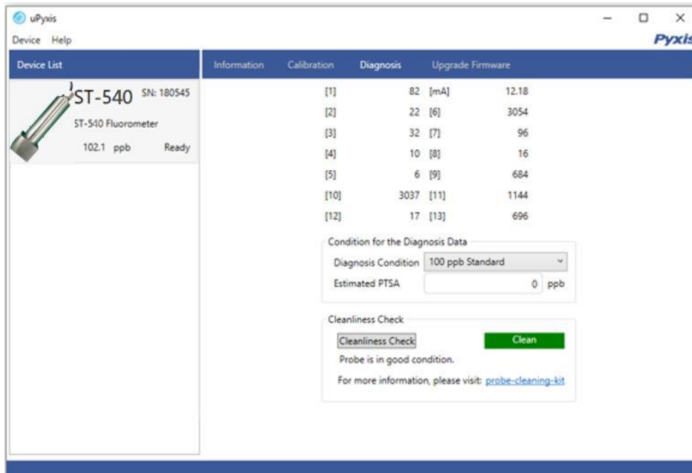
Figure 16. Cleanliness check and raw diagnosis data
