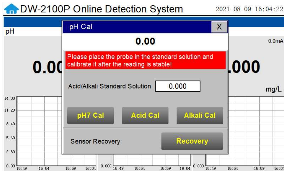
Figure 17 pH Calibration
