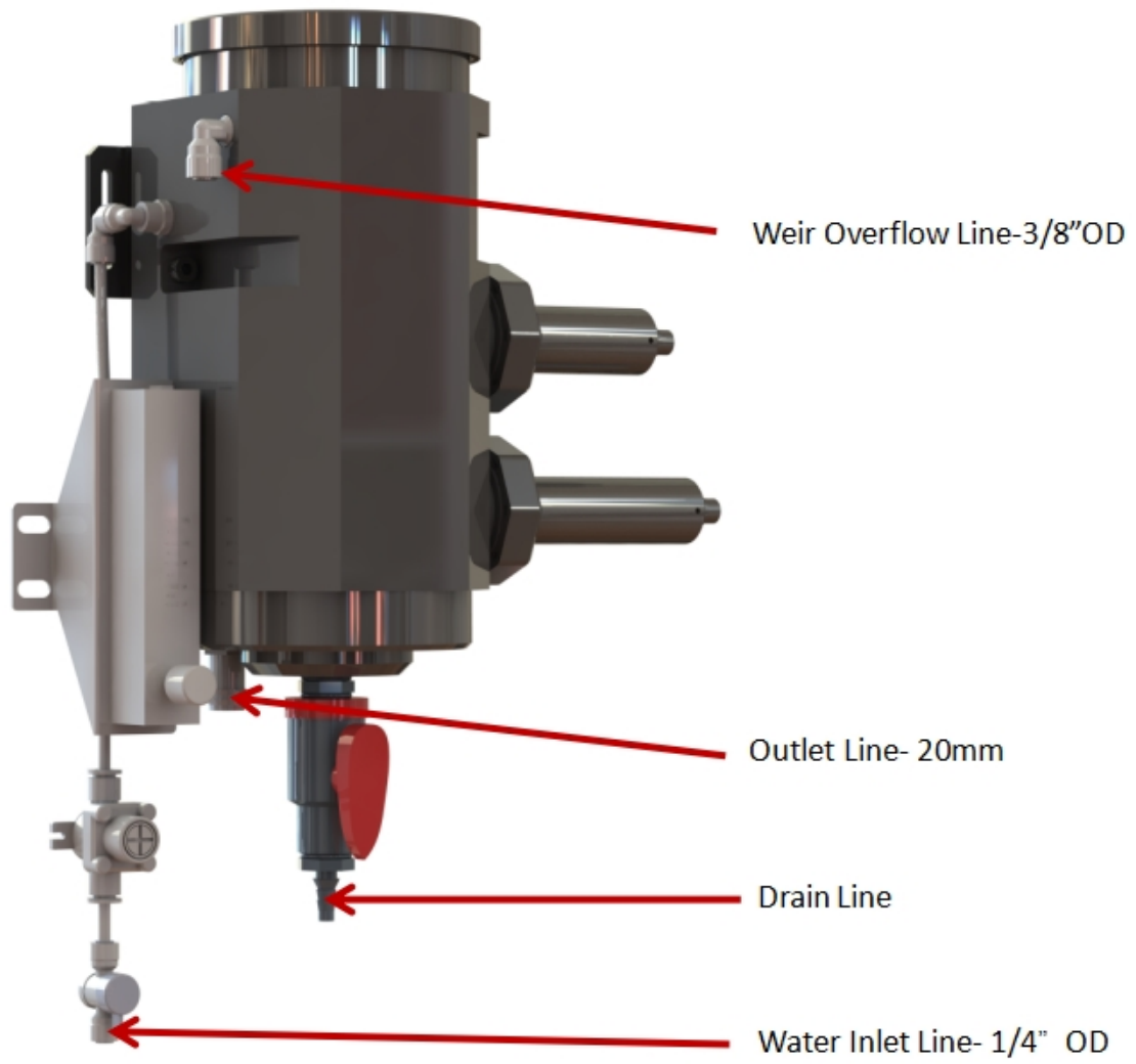
Figure 2 FR-200 Connections
