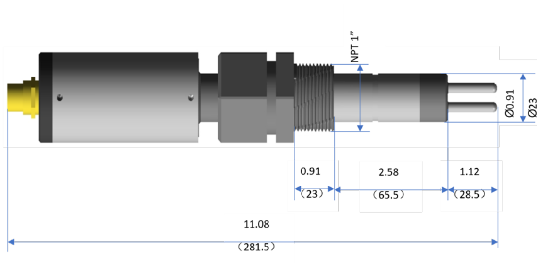
Figure 4. CR-300 Series Dimensions in inch (mm)
