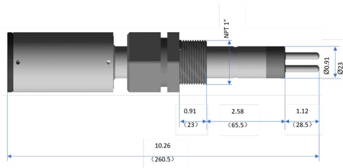
Figure 3. CR-200 Series Dimensions in inch (mm)
